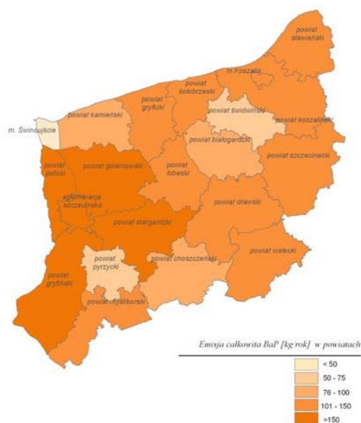
d) benzo(a)piren
